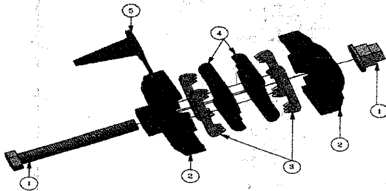
VISTA EXPLODIDA
